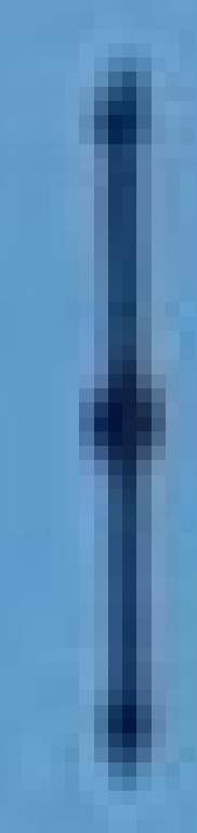
Linearly polarized or plane-polarized light
